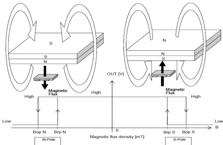
Figure 3, Magnetic Operation Characteristic of AS1826A
