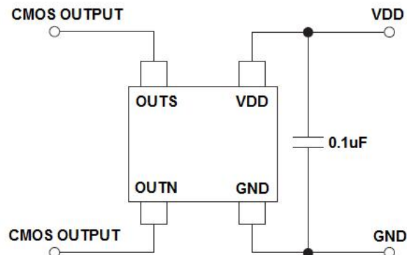
Figure 1, Typical Application Circuit of AS1826A
