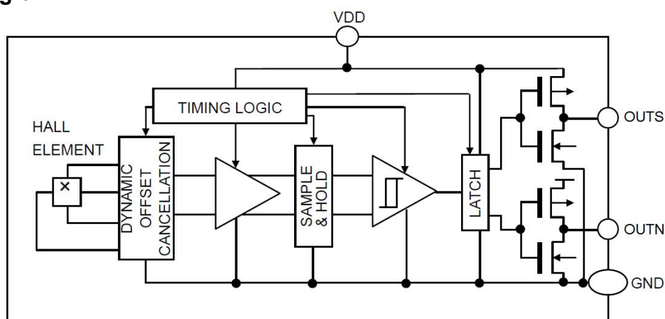
Figure 2, Block Diagram of AS1826A
